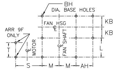
FOUNDATION PLAN MOTOR LOCATION 'L' (LEFT) SHOWN
