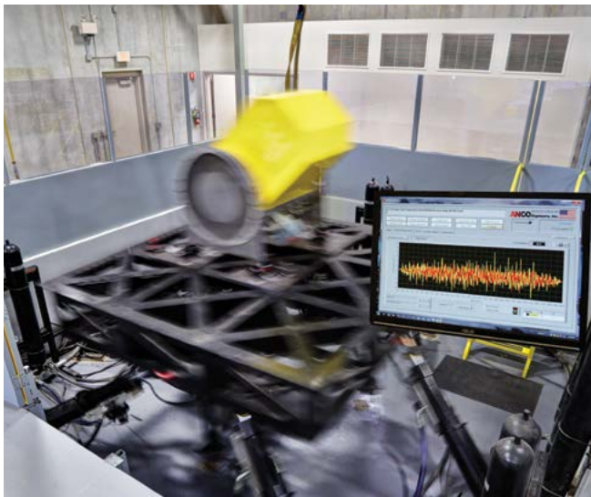
Twin City Fan & Blower's State-of-the-Art Shaker Table
